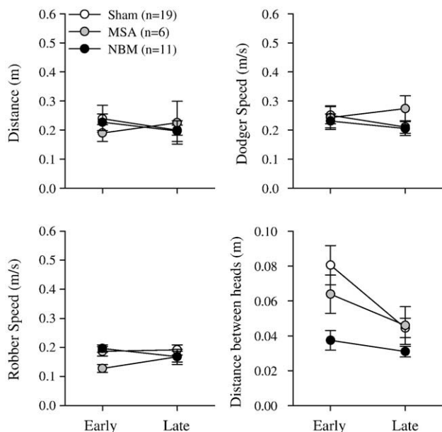
Fig. 6 – Several measures were used to characterize each group's bracing behavior observed during early and late samples: average distance traveled by the dodger (top left panel), average speed of the dodger (top right panel), average speed of the robber (bottom left panel), and average distance between heads at the start of a dodge (bottom right panel). Note: the number of subjects reflects the rats that exhibited bracing behavior in both samples.
